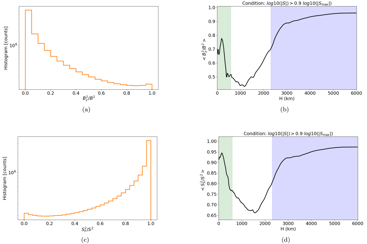
Figure 4. Left panels: distribution of B_z^2/B^2 (panel (a)), and the distribution of the ratio S_h^2/S^2 (panel (c)) from the solar surface up to a height of 390 km. Right panels: average value of B_z^2/B^2 (panel (b)) and S_h^2/S^2 (panel (d)) for regions where \log_{10}(|S|) > 0.9\log_{10}(S_{max}) as a function of height. The colors indicate the average height range of the photosphere (green), chromosphere (white), and transition region and corona (purple).
