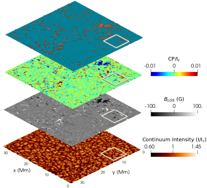
Figure 2. From bottom to top: IMAx continuum intensity, magnetic field obtained from SPINOR inversions saturated at 100 G, IMAx CP maps and magnetic elements depicted in orange. The white box indicates the sub-FOV shown in Fig. 6.
