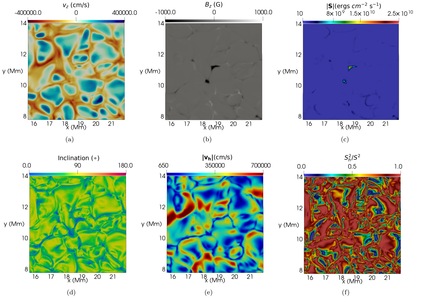
Figure 3. Close view of a 6.25 \times 6.25 Mm 2 region from the Bifrost simulation indicated by the white rectangle in Fig. 1. The horizontal planes are placed \sim 115 Km above the solar surface. The individual panels illustrate: (a) the vertical component of the velocity field, (b) vertical component of the magnetic field, (c) the magnitude of the Poynting flux, (d) the inclination of the magnetic field, (e) the horizontal plasma velocity and (f) the ratio S_h^2/S^2 .
