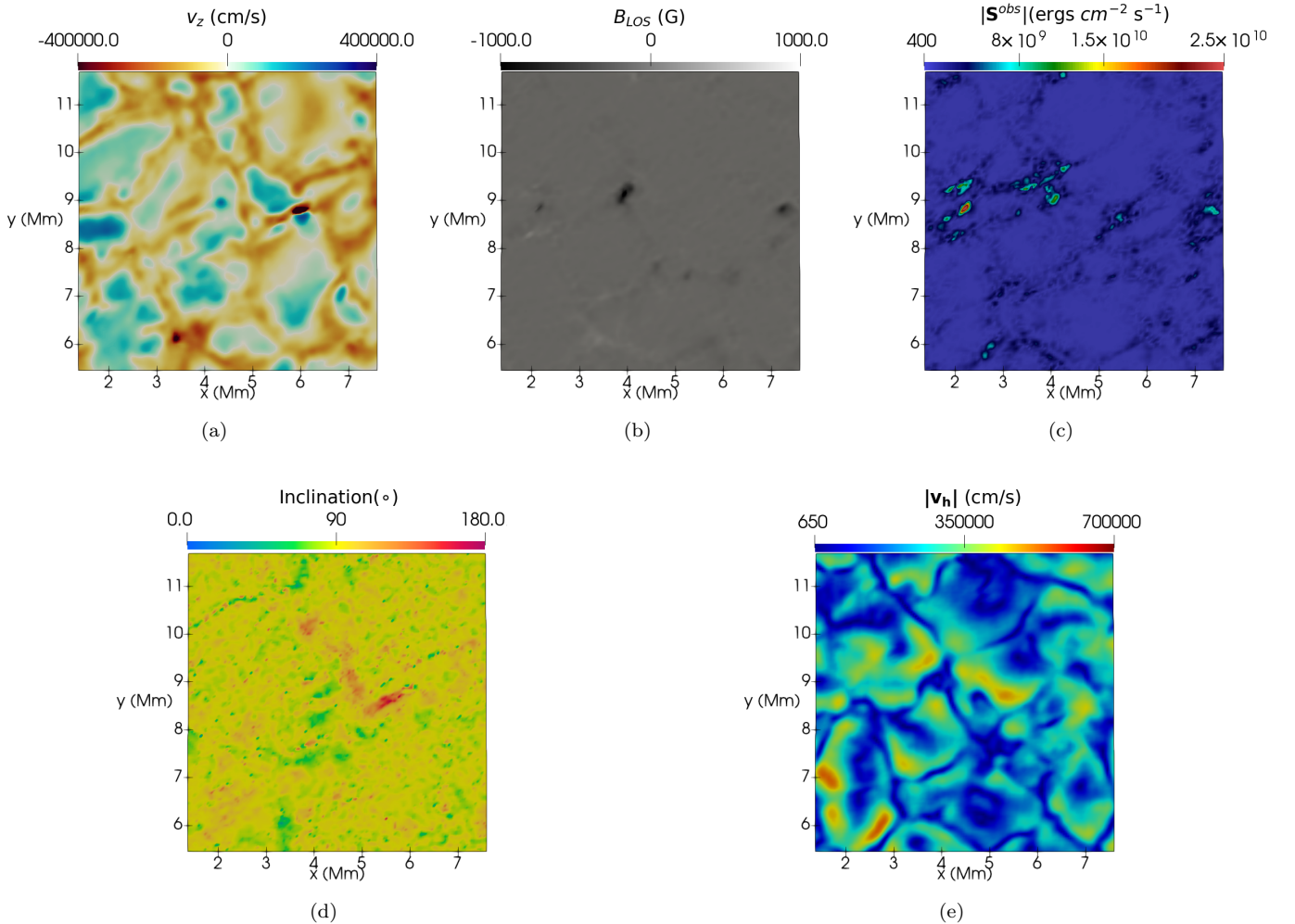
Figure 6. Close view of a \sim 6.2 \times 6.2 \text{ Mm} region from the IMaX observation indicated by the white rectangle in Fig. 2. (a) the vertical component of the velocity field; (b) the vertical component of the magnetic field, (c) the magnitude of the proxy of the Poynting flux; (d) the magnetic field inclination; (e) the horizontal plasma velocity.
