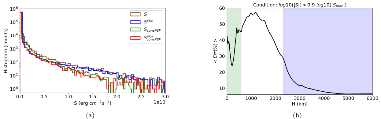
Figure 5. (a) Distribution of the Poynting flux derived from the simulation as described by Eq. 3 (blue histogram) and with the approximation (brown distribution) using the Eq. 5. The red/green distributions have been obtained by convolving the original simulation with the IMAx PSF. (b) Average value of the relative error, Err , for regions where \log_{10}(|S|) > 0.9 \log_{10}(S_{max}) as a function of height.
