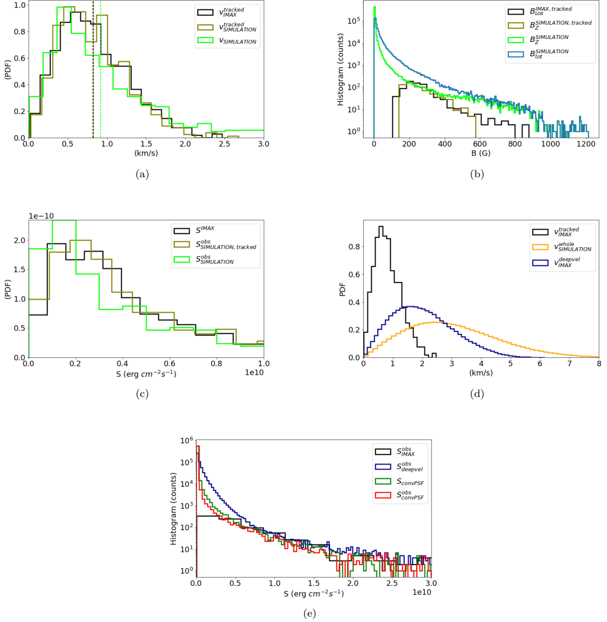
Figure 7. (a) Probability density function of the horizontal velocity field, v_h , associated with the magnetic elements tracked in the IMAx data (black histogram) and the simulation domain (olive histogram). The green distribution represents v_h derived from the simulation at 115 km at the same magnetic elements selected. The three dashed lines indicate the average values of v_h . (b) Distribution of the vertical magnetic field at the magnetic elements in the IMAx (black histogram) and the simulation (olive histogram) data sets. For comparison, considering all pixels of the simulation domain at 115 km (i.e. photospheric heights), we also show B_z and the total magnetic field (green and light blue histograms). (c) Probability density function of the horizontal Poynting flux calculated by means of Eq. 5. (d) Overview of the horizontal velocity of the IMAx data (derived with two methods; black and blue histograms) and for the simulation (orange histogram). (e) Distribution of the total Poynting flux using the Eq. 4 ( S_{convPSF} , green histogram), and the Poynting flux derived using Eq. 5 ( S_{convPSF}^{obs} , red curve). Both quantities are convolved with the IMAx PSF. The black histogram represents the Poynting flux as derived from the IMAx observations, and the blue curve shows the Poynting flux using the value of v_h retrieved with the Deepvel method for the IMAx data.
